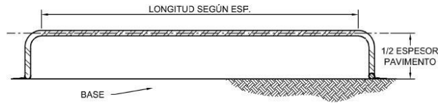
VISTA (C)
