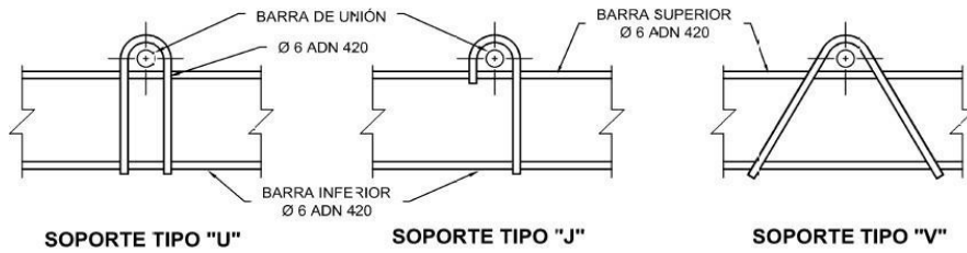
DETALLE (C) SOPORTES
